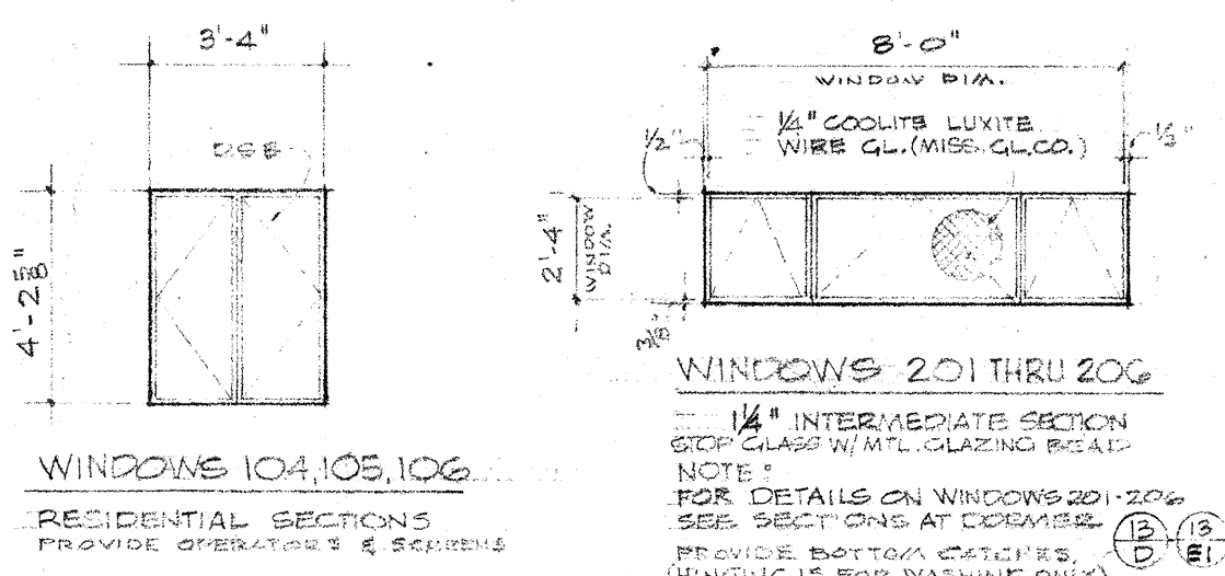
WINDOW ELEVATIONS SCALE 3/4" = 1'-0"
