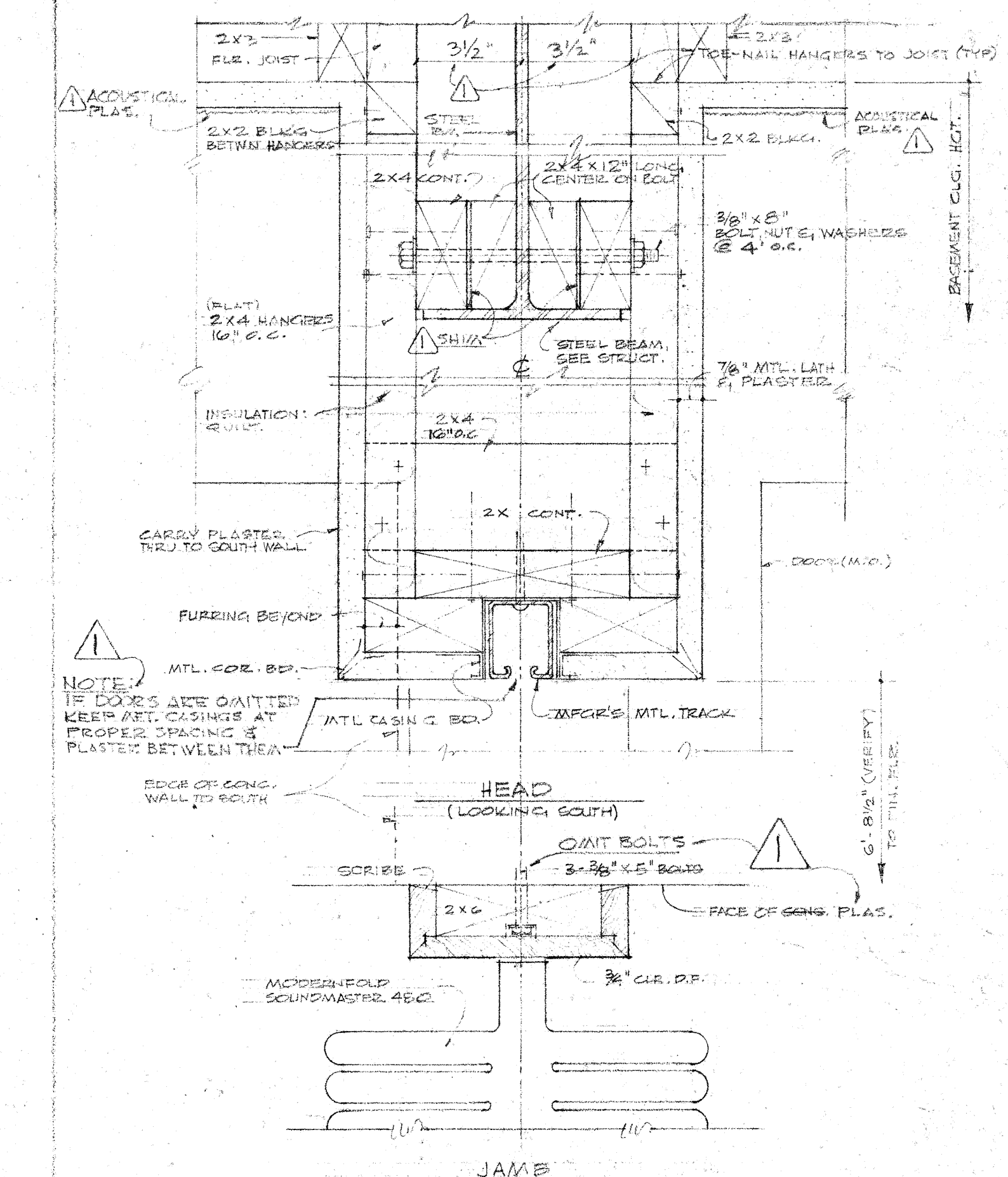
MODERNEFOLD FOLDING PARTITIONS SCALE: 3/4" = 1'-0"
