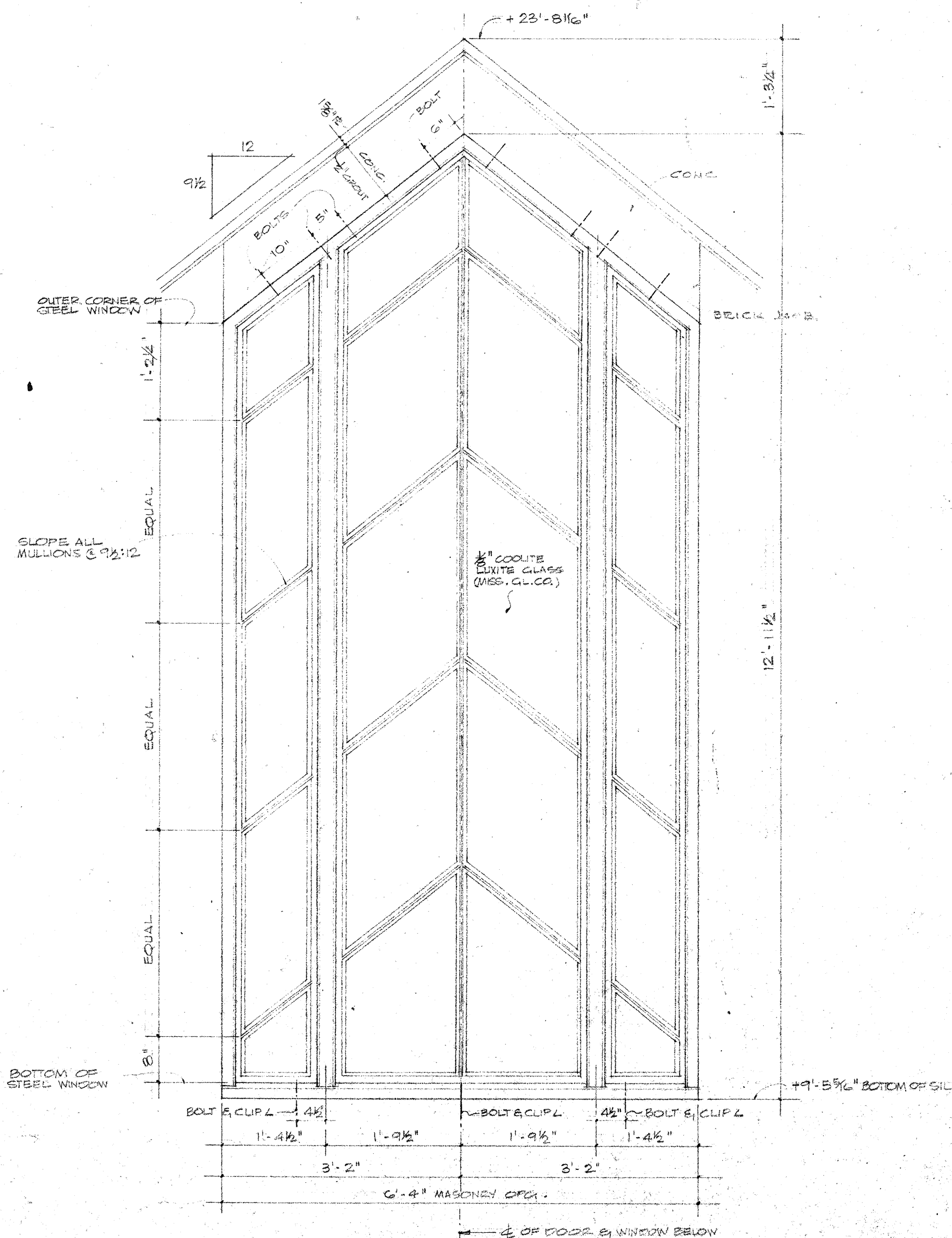
1/4" INTERMEDIATE SECTIONS (STEEL)
